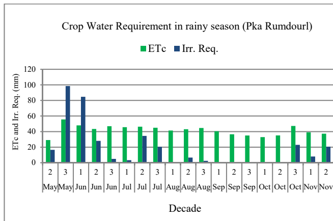
Fig.4. Graph of water requirement and crop needs irrigation (CROPWAT Data)
