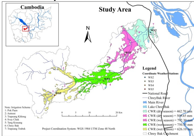
Fig.6. Crop water requirement of rice in Chrey Bak catchment
