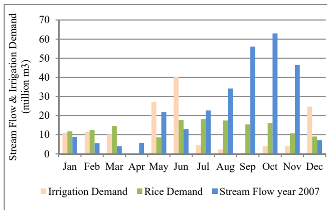
Fig.8. Comparison of monthly stream flow, rice demand & irrigation demand
