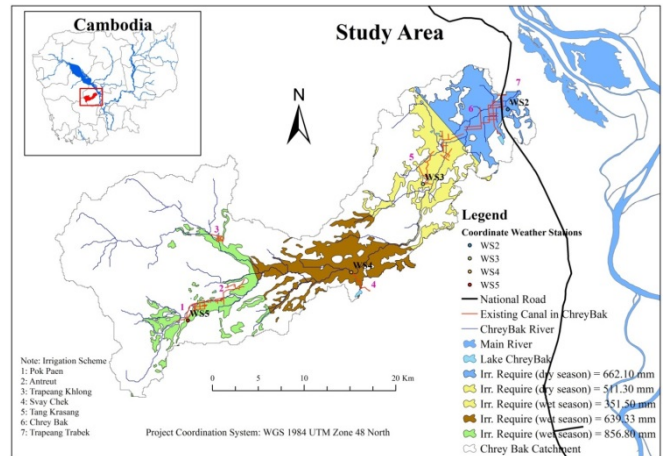
Fig.7. Irrigation requirement of rice in Chrey Bak catchment
